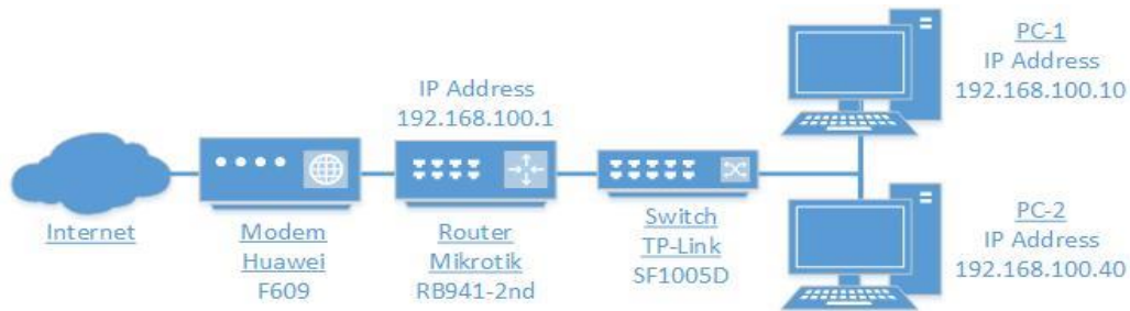
Figure 7. The network topology of static and dynamic alliance
