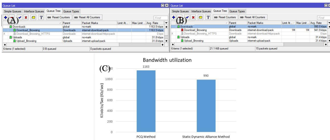
Figure 11. (A) The WinBox shown bandwidth utilization of PCQ method was above 1 Mbit/sec; (B) The WinBox shown bandwidth utilization of Static and Dynamic Alliance method was below 1 Mbit/sec; (C) The summary of WinBox indicated Static and Dynamic Alliance method were capable to reduce bandwidth utilization to below maximum bandwidth value of 1 Mbit/sec.
